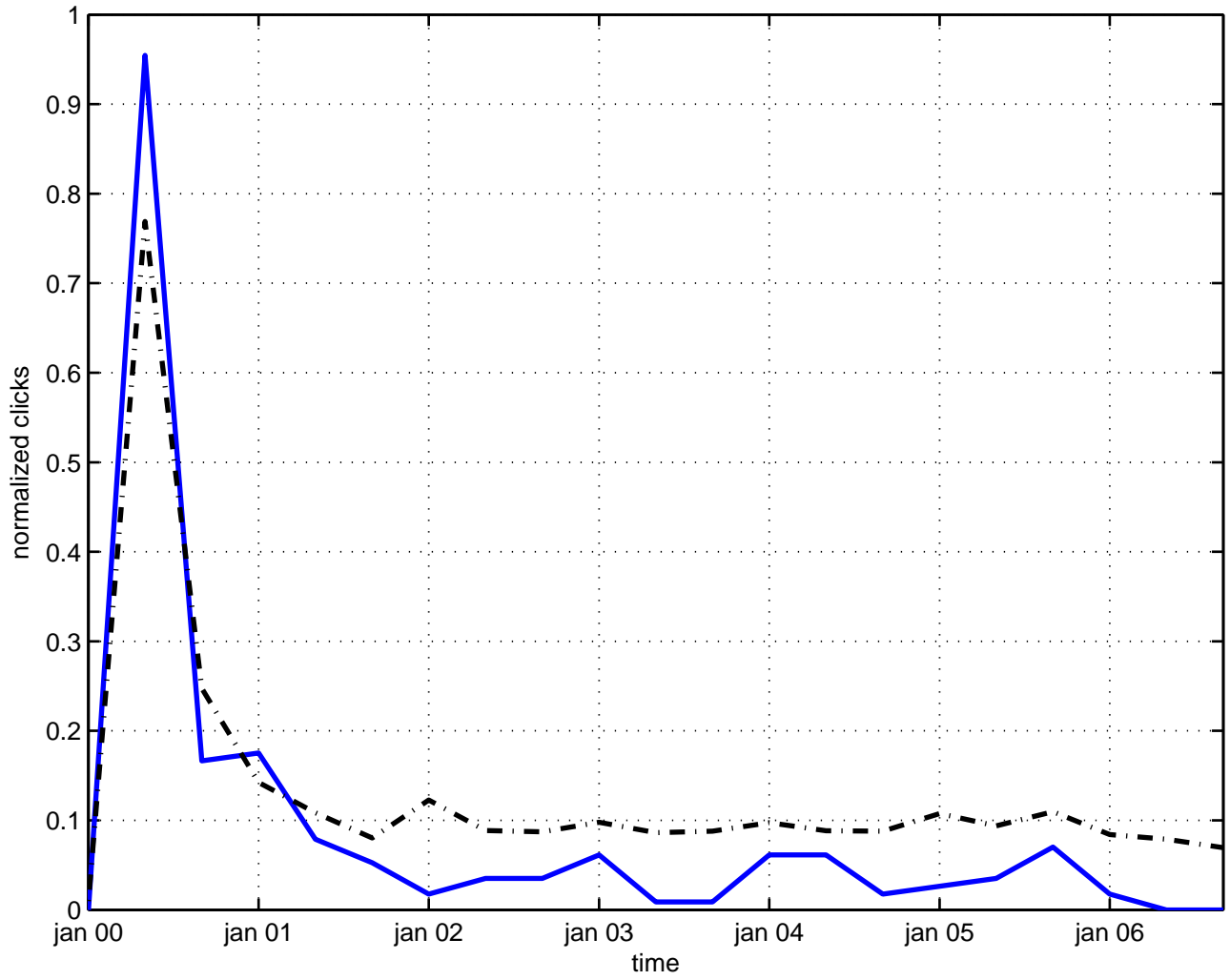
t(4) space-time
