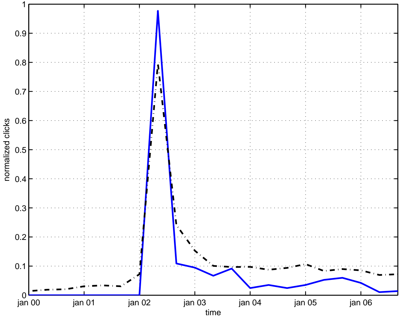
t(3) spontaneous compactification
