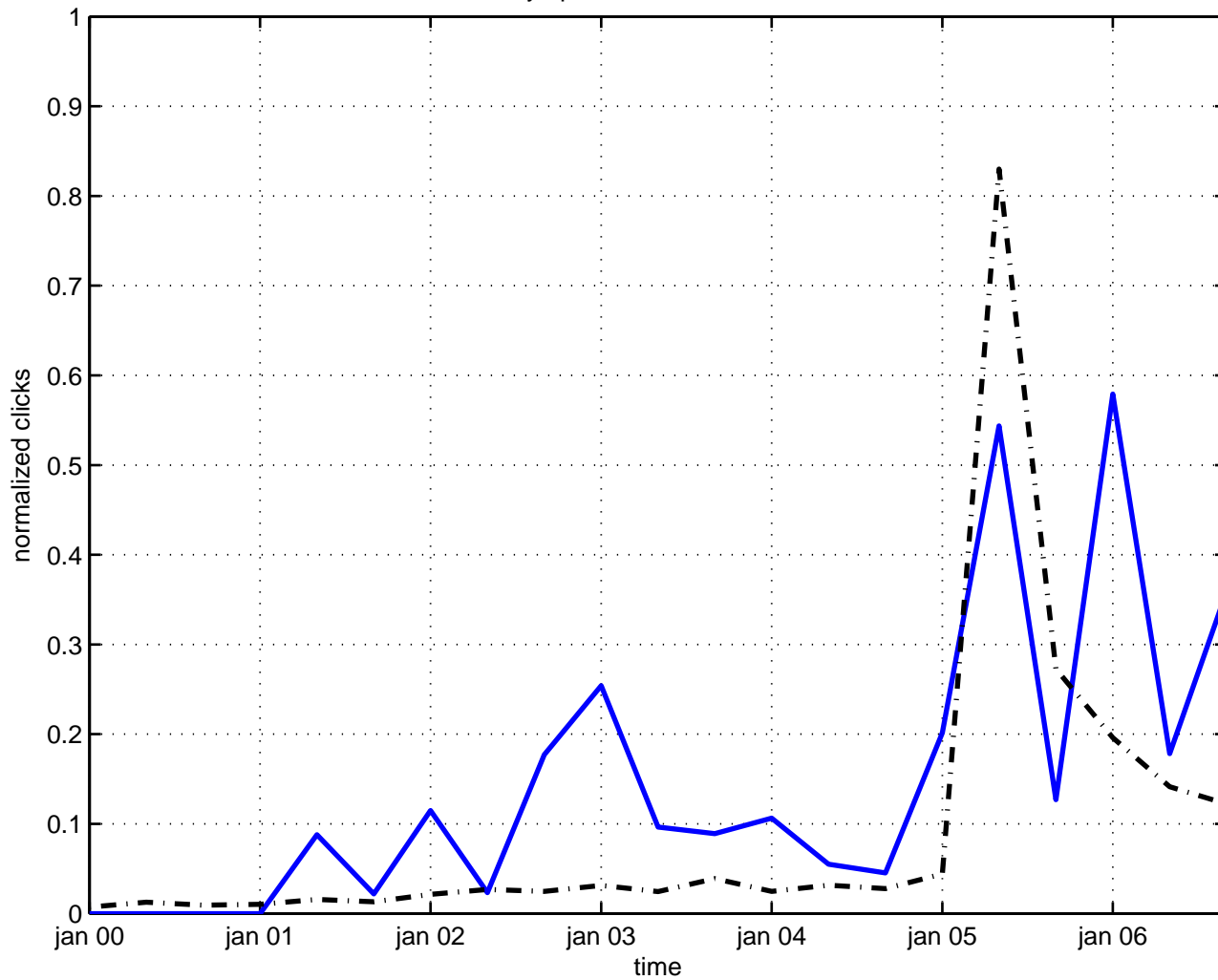
symplectic transformation
