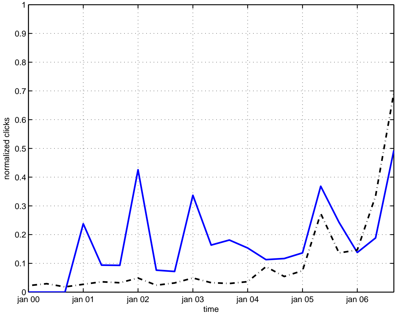
symplectic geometry
