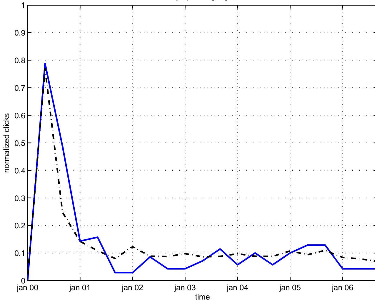
symplectic gauge
