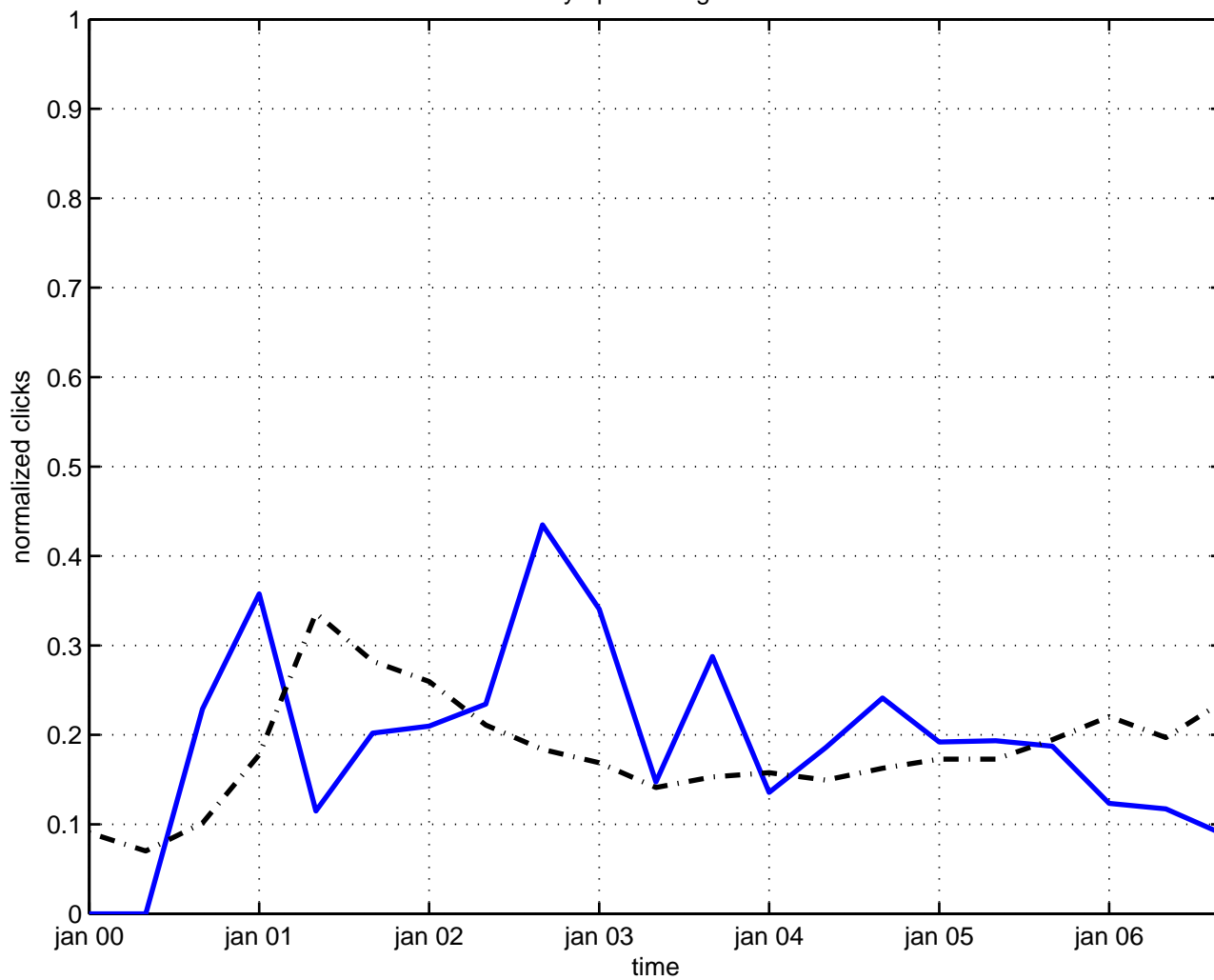
symplectic algebra
