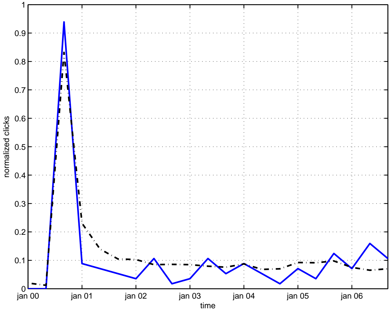
symmetry transformation
