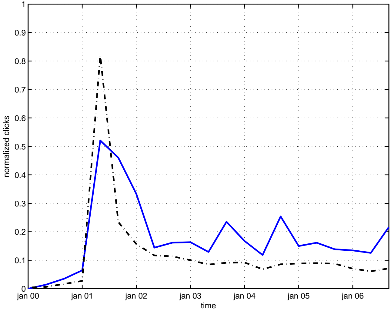
symmetry space-time
