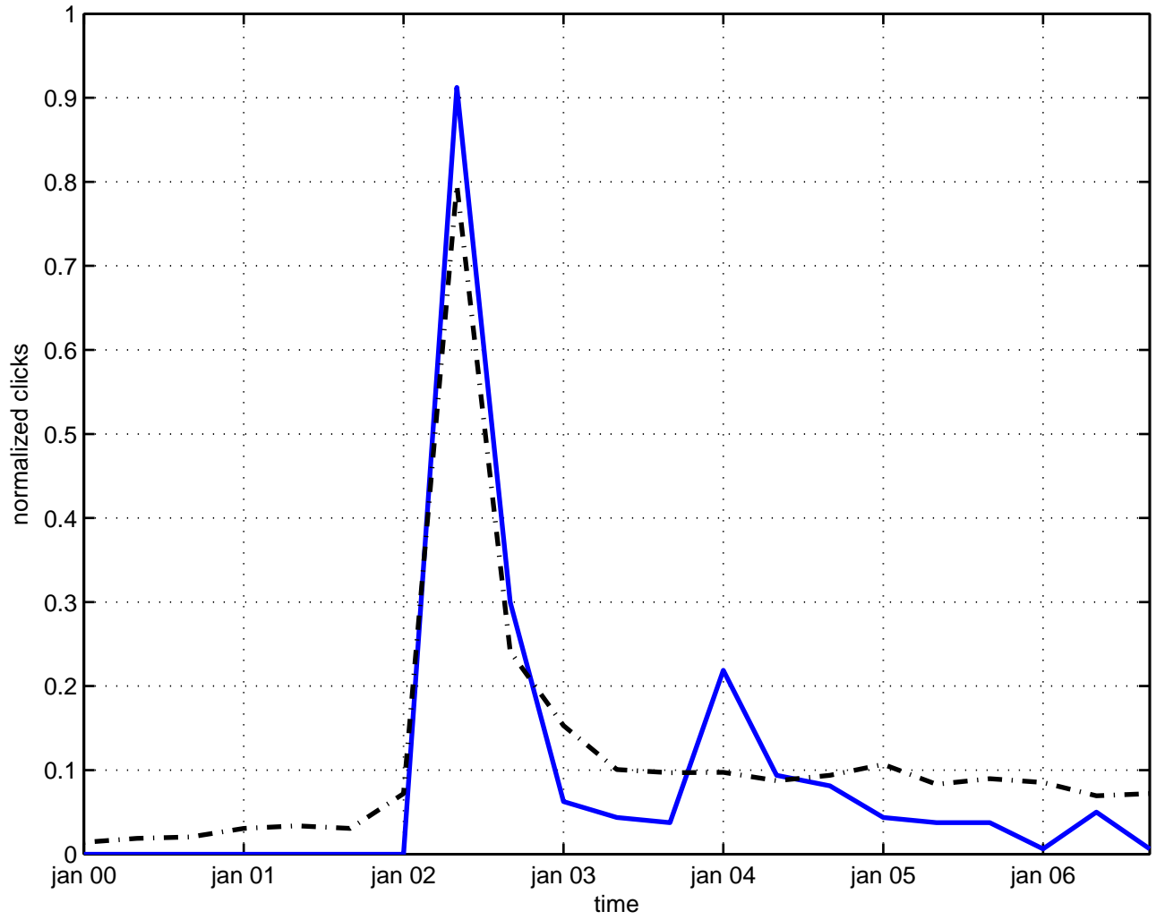
symmetry particle antiparticle
