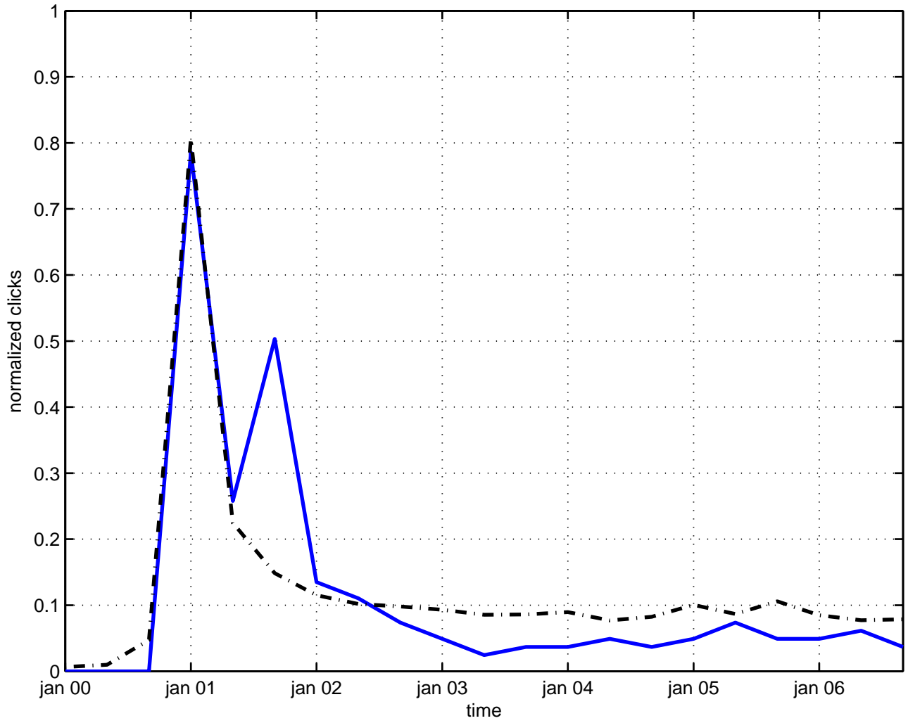
symmetry fermion
