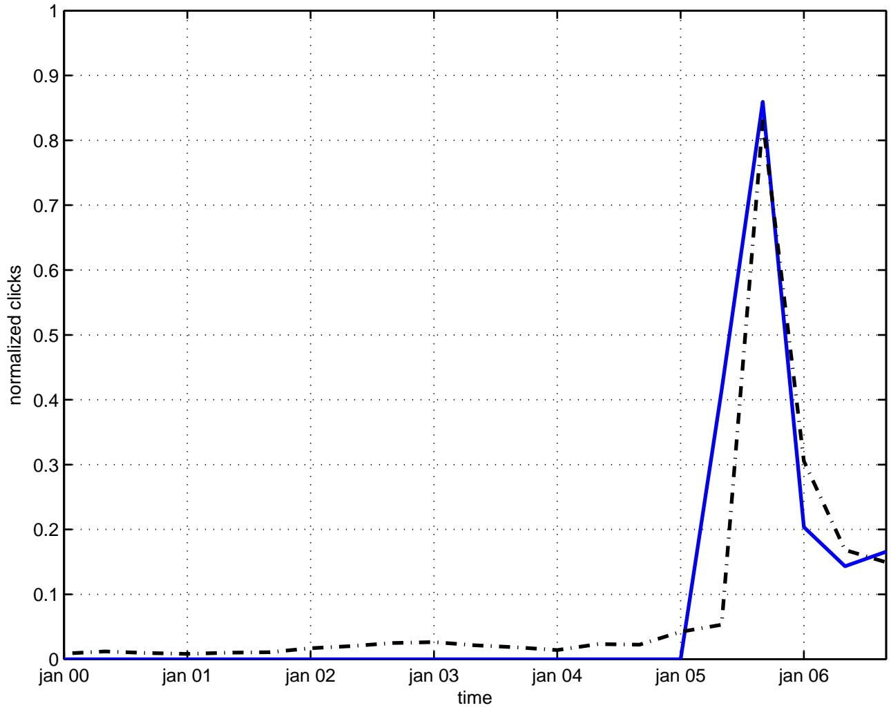
symmetry breaking hidden symmetry
