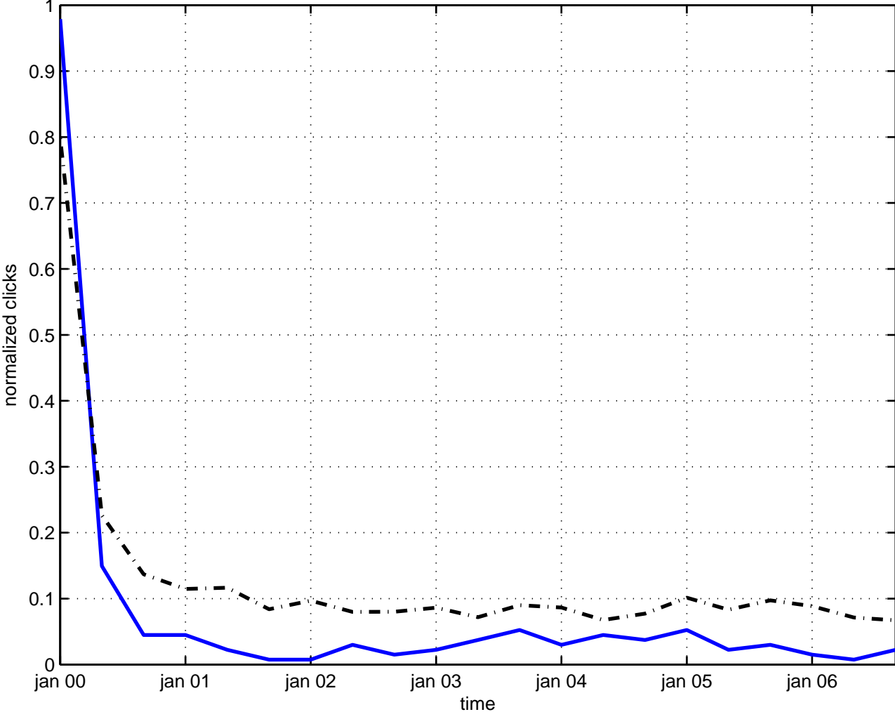
surface space-time
