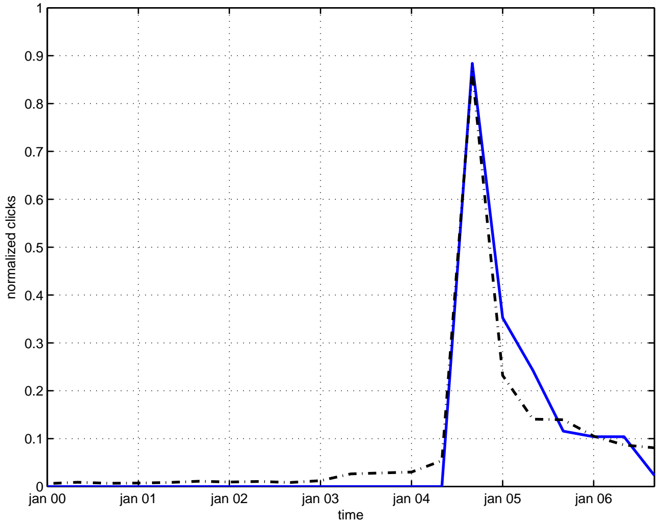
supertube tachyon
