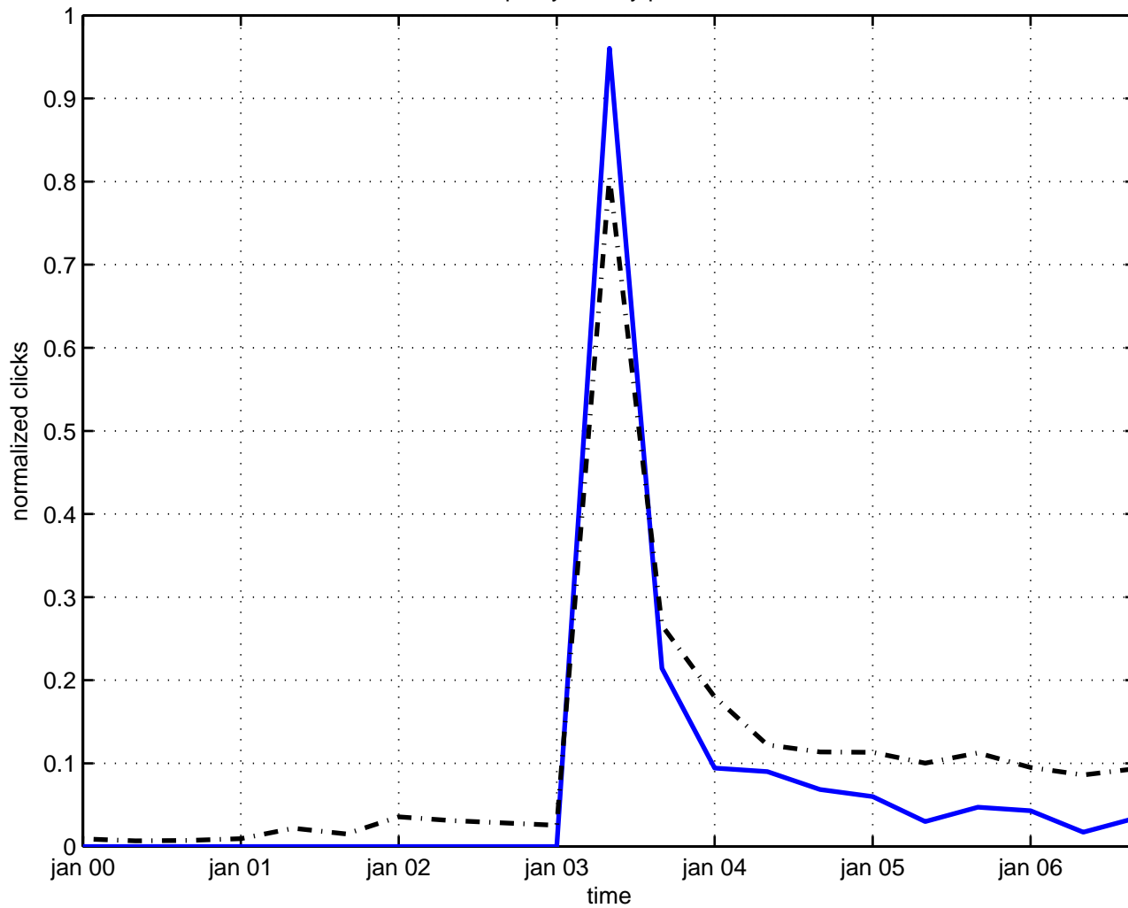
supersymmetry potential
