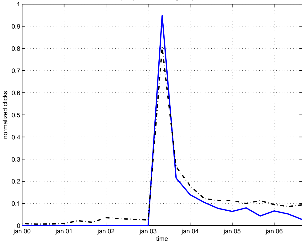
superspace schroedinger equation
