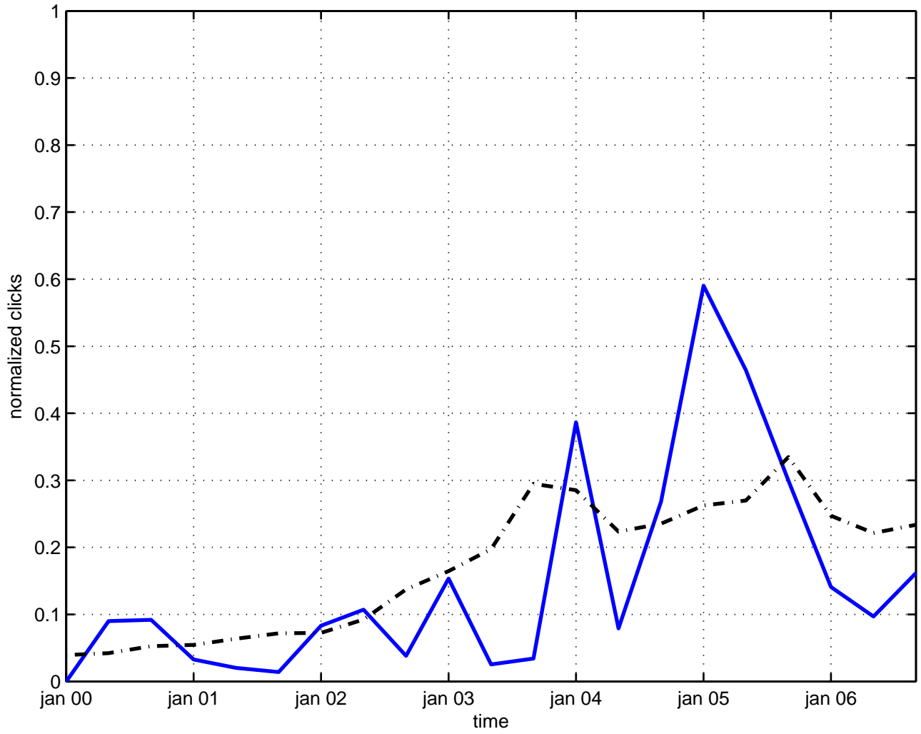
superselection rule
