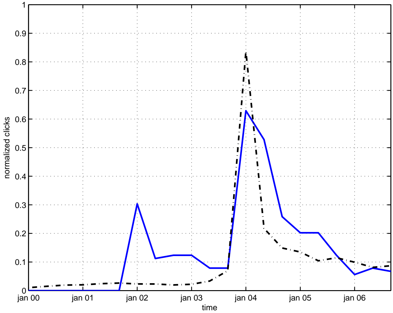
superselection rule charge
