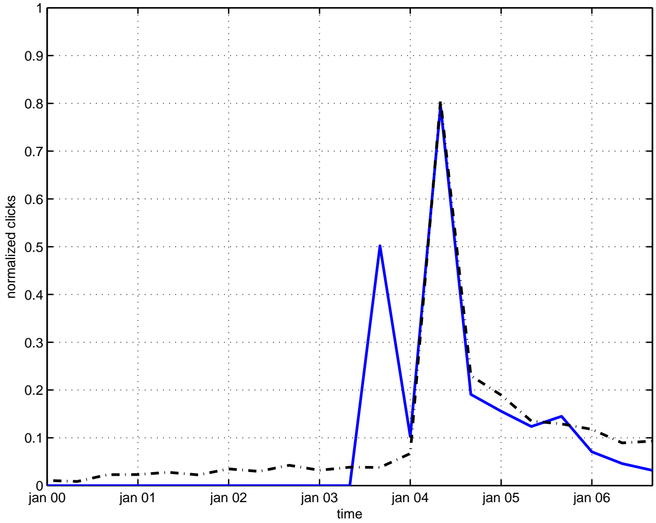
superpotential supersymmetry
