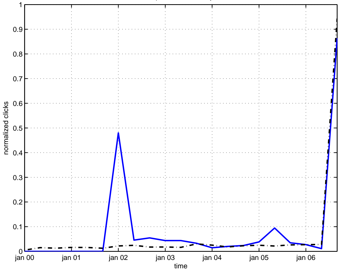
superluminal velocity
