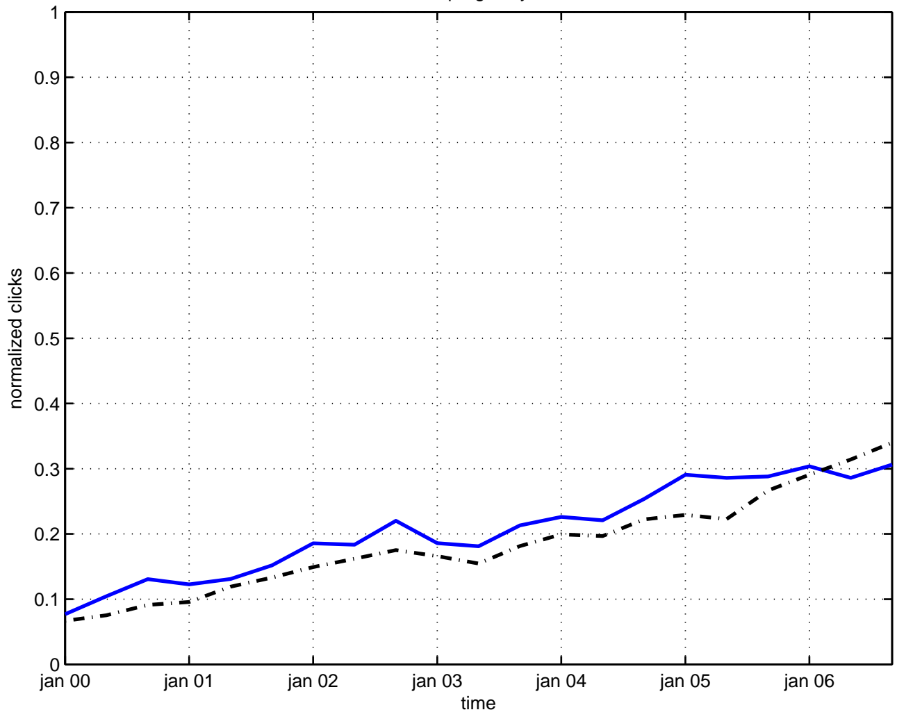
supergravity
