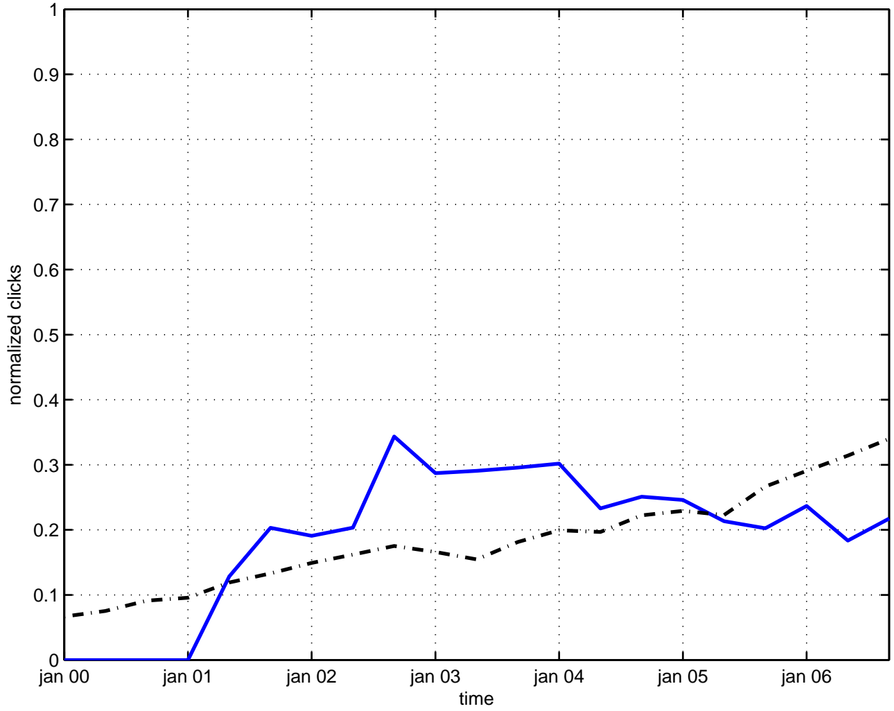
supergravity supersymmetry
