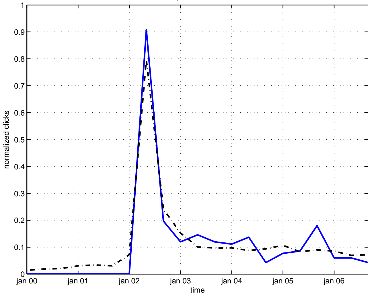
superfluid helium
