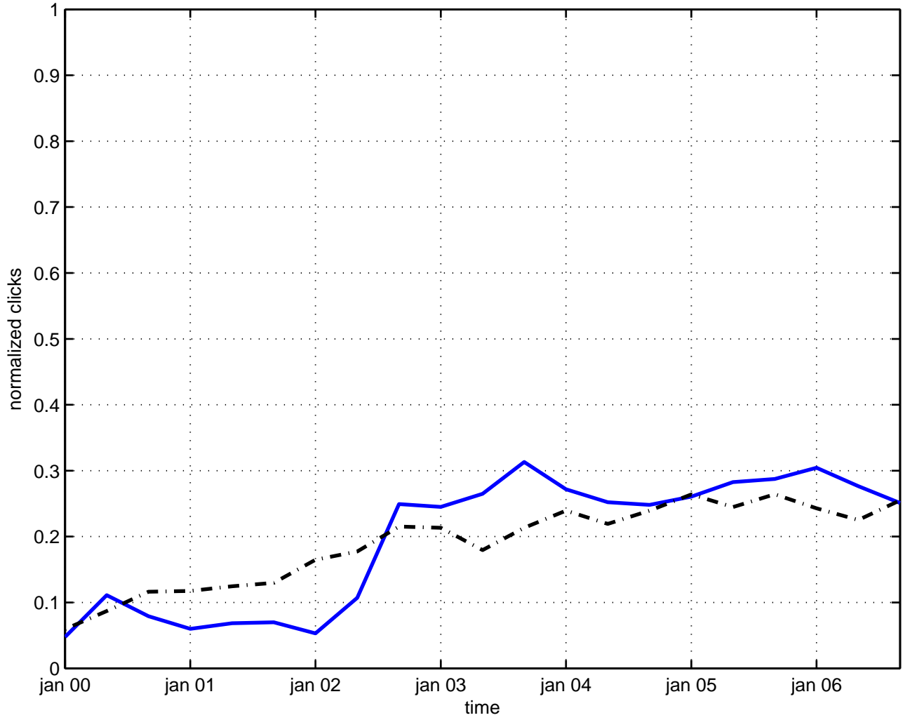
superfield supersymmetry
