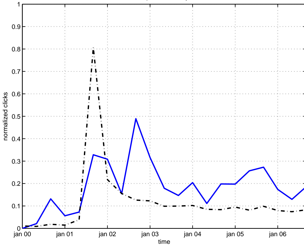
superconductivity
