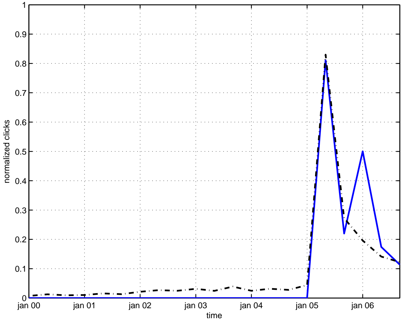
superconductivity vortex
