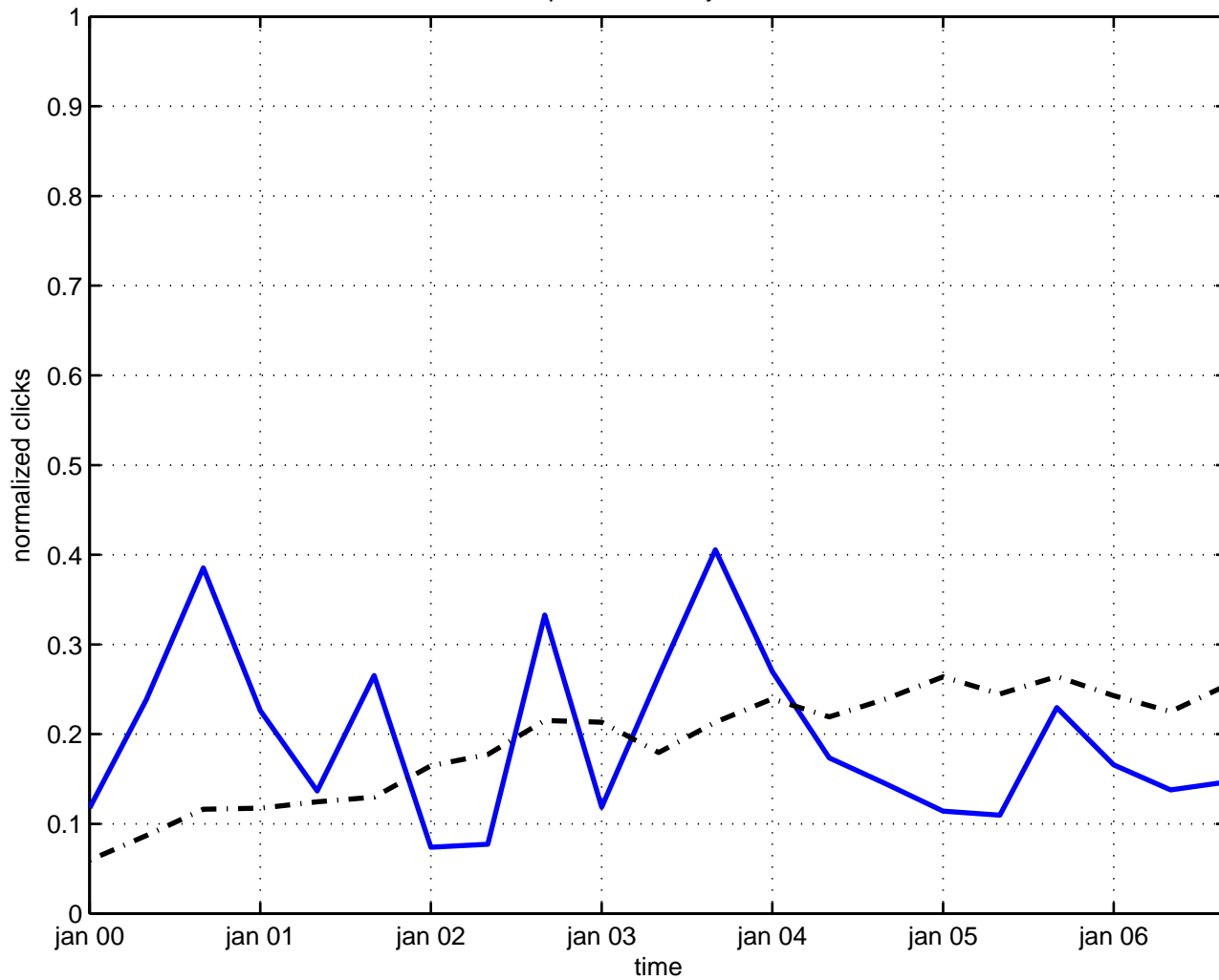
superconductivity model
