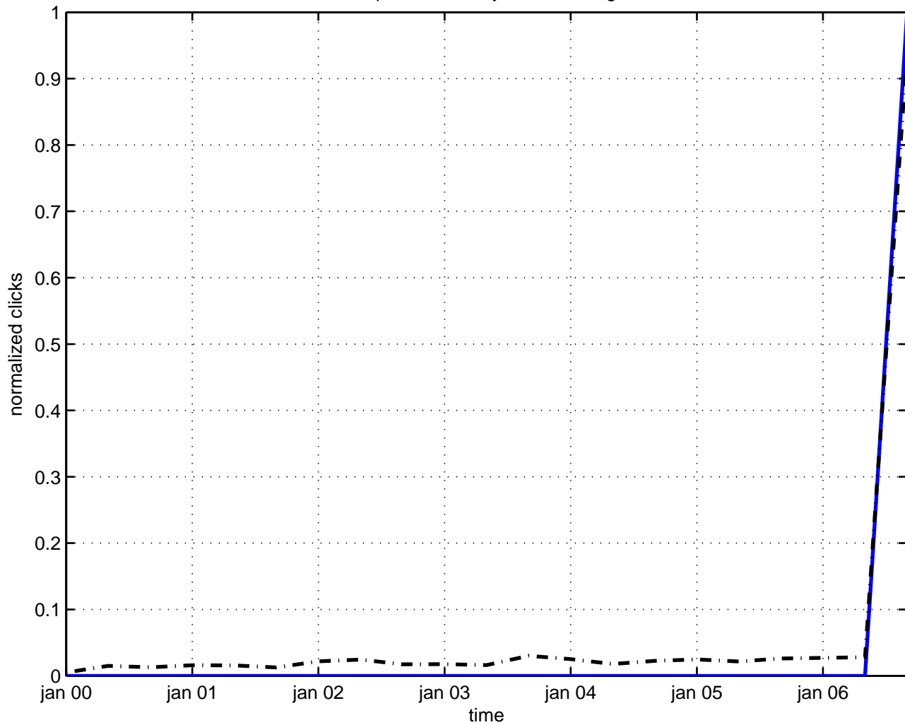
superconductivity cosmic string
