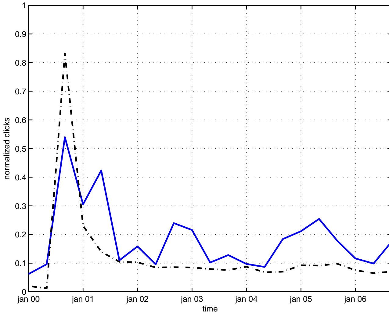
sum rule
