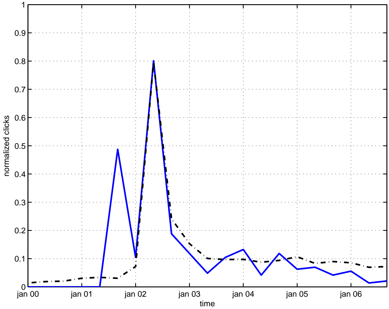
sum rule anomaly
