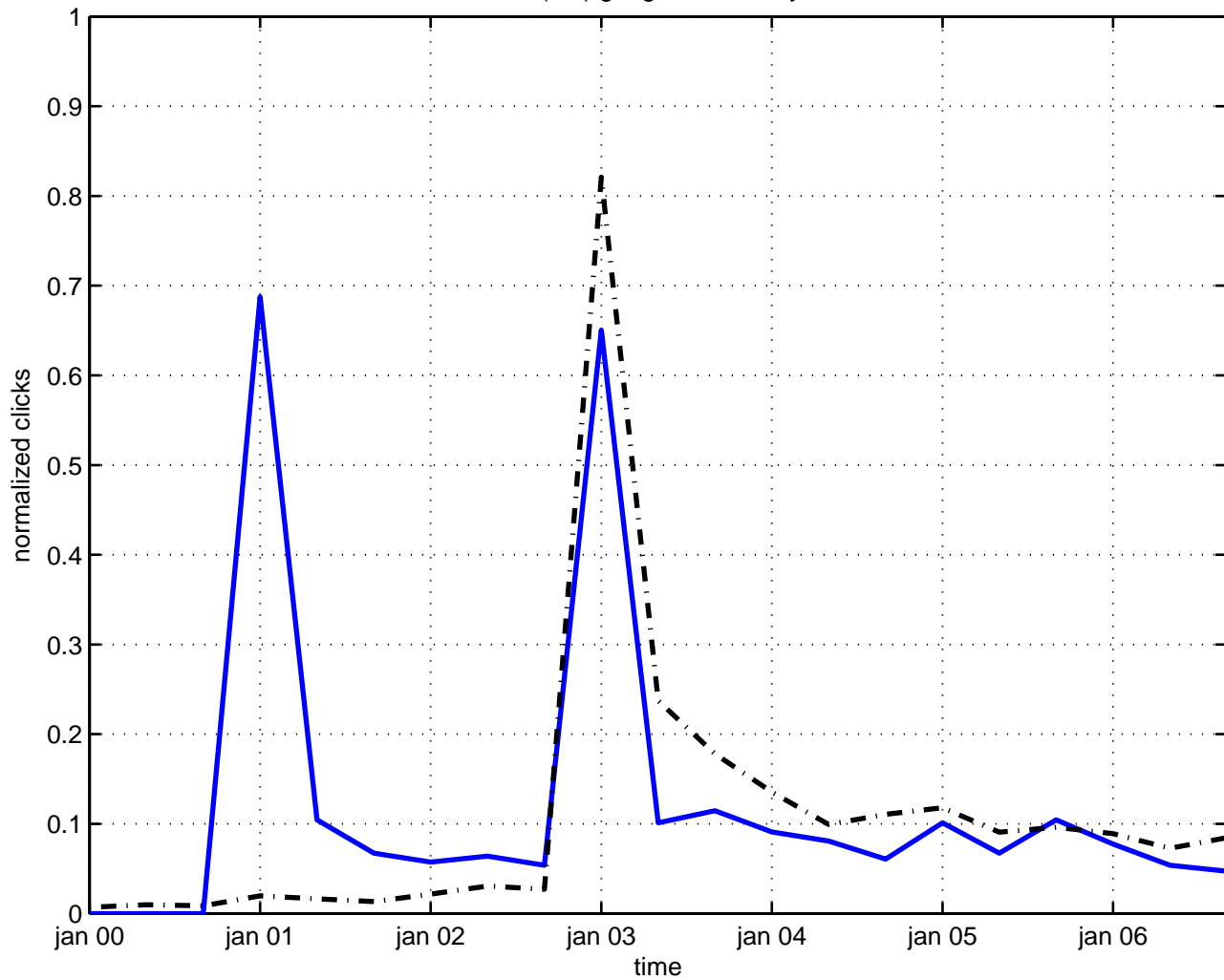
su(n/n) gauge field theory
