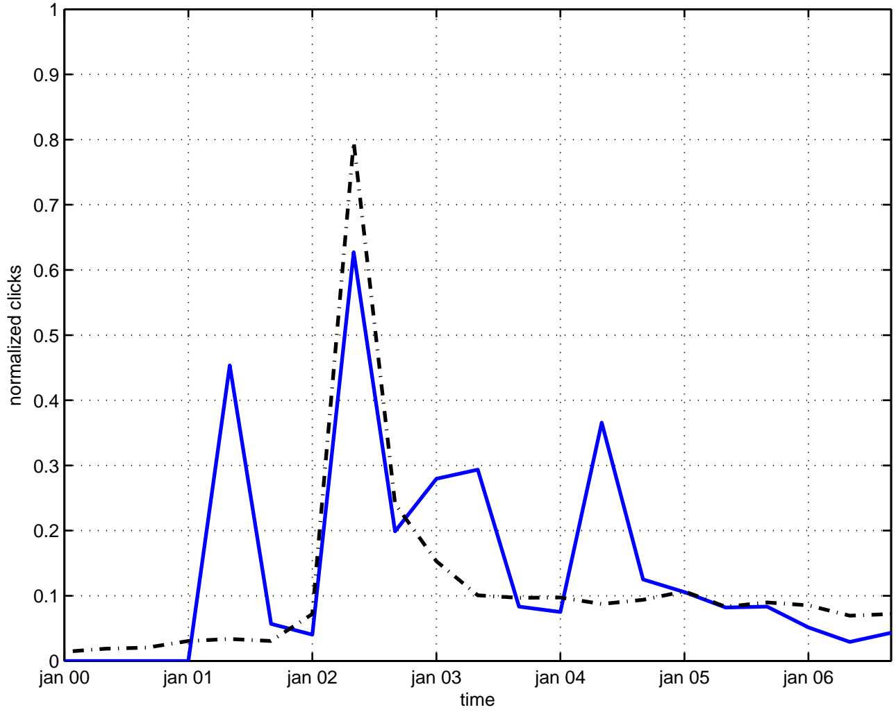
su(n)**m gauge field theory
