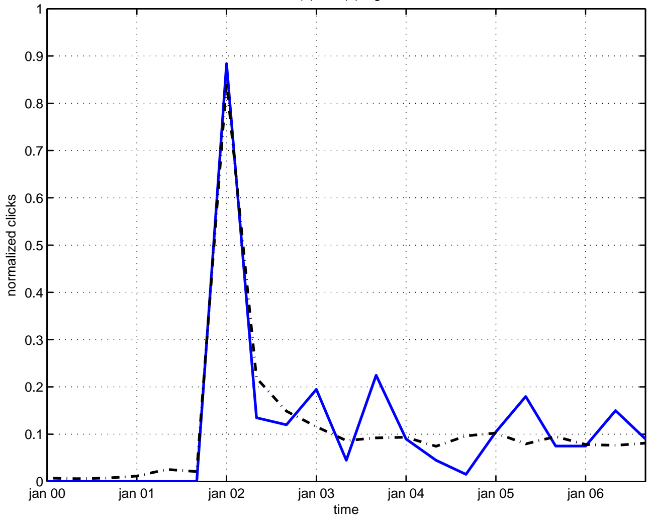
su(n) x su(n) algebra
