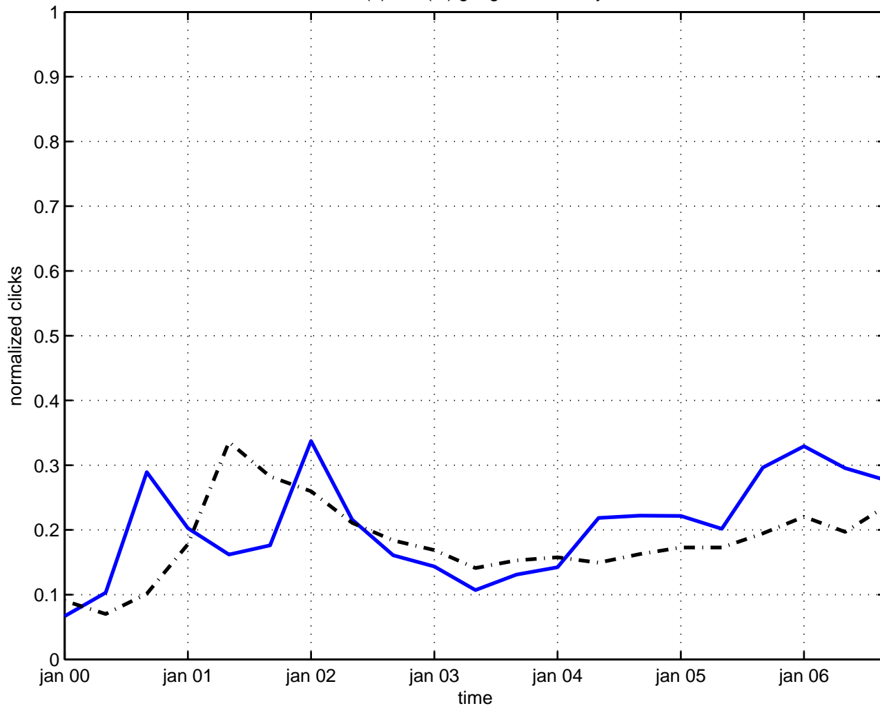
su(n) x su(m) gauge field theory
