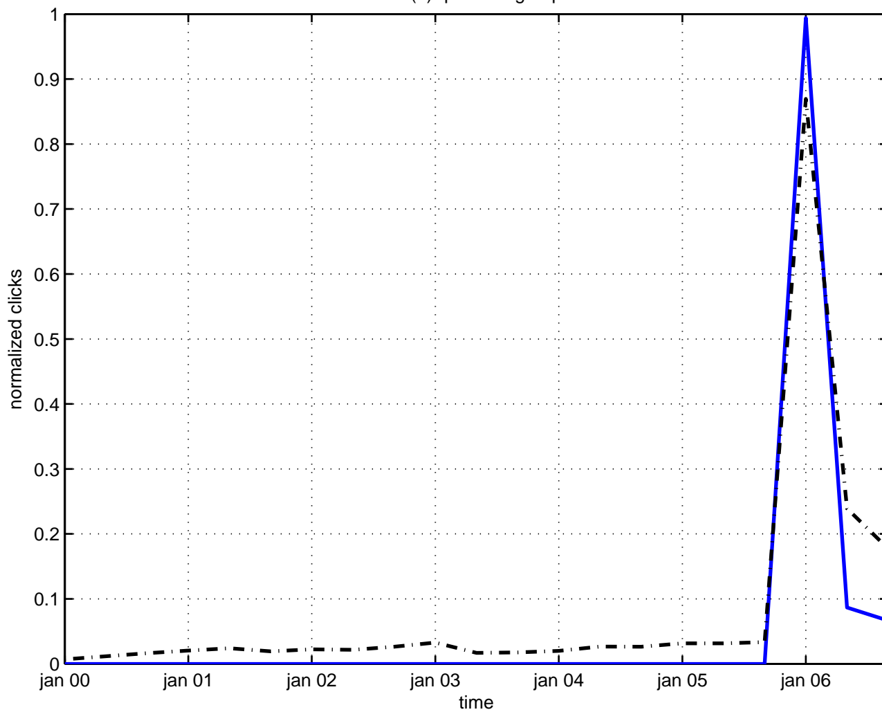
su(n) quantum group
