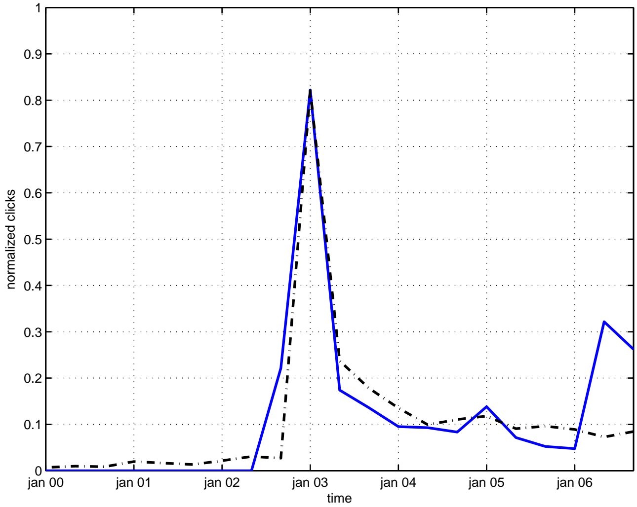
su(n) holonomy
