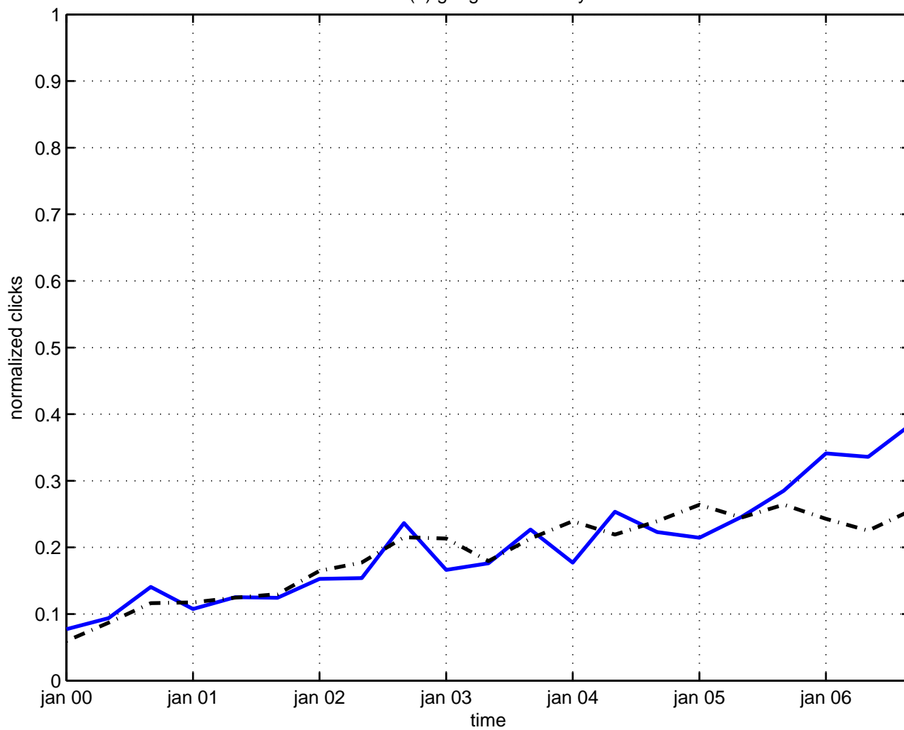
su(n) gauge field theory
