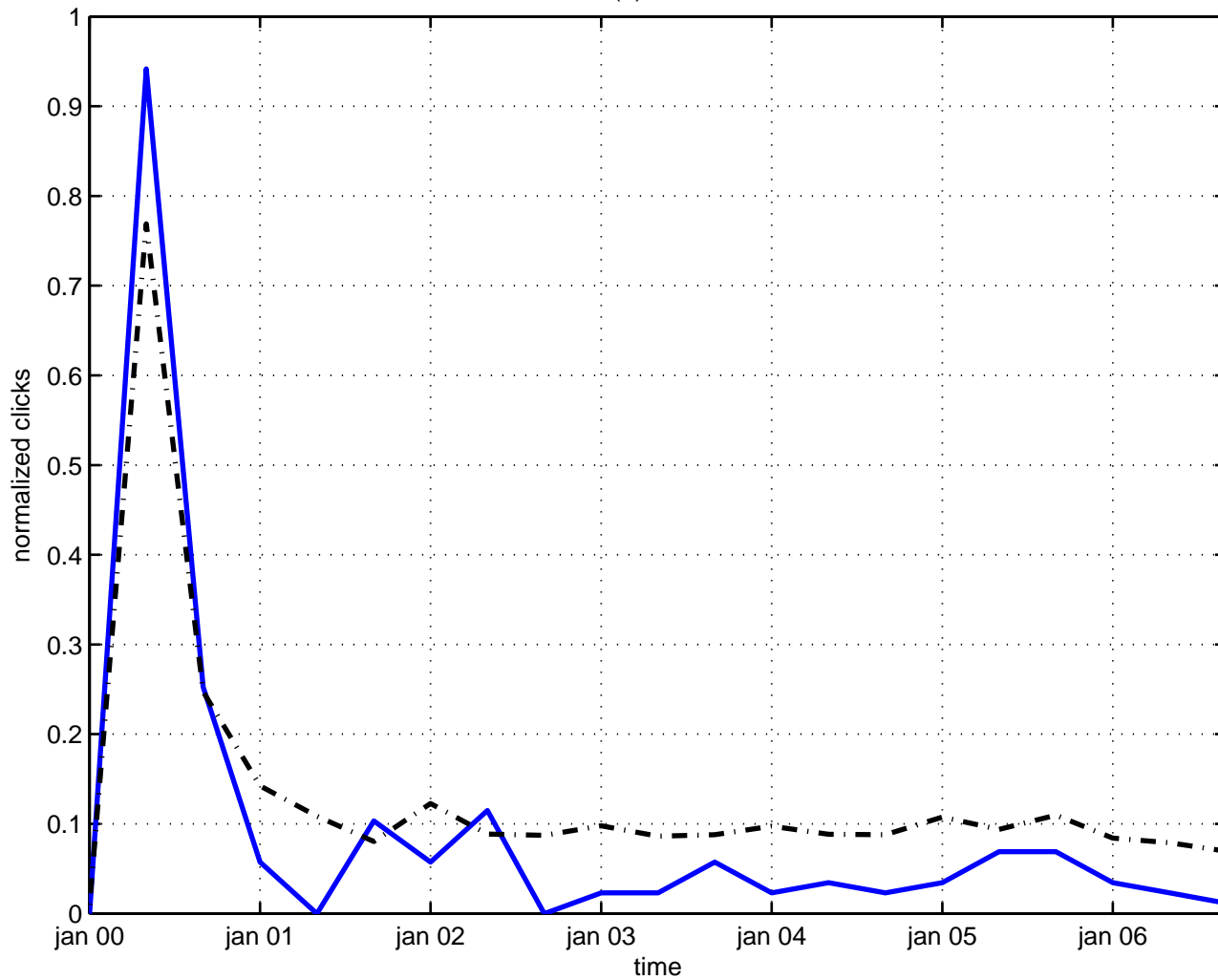
su(n) current
