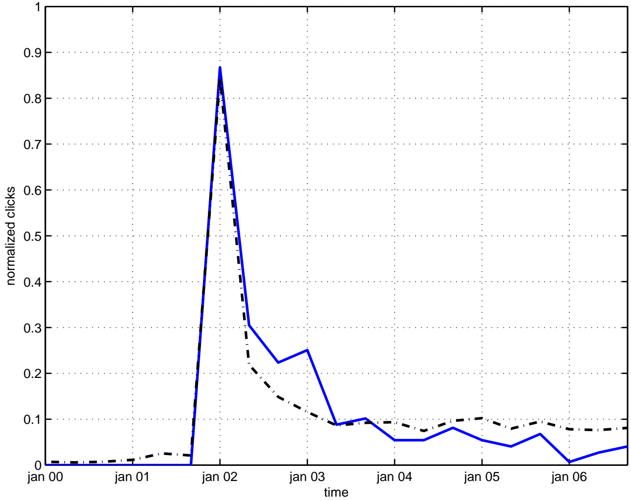
su(5)**n grand unified theory
