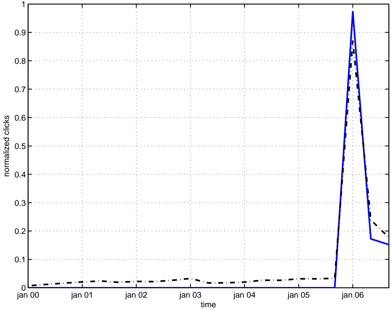
su(5) x z(2) grand unified theory
