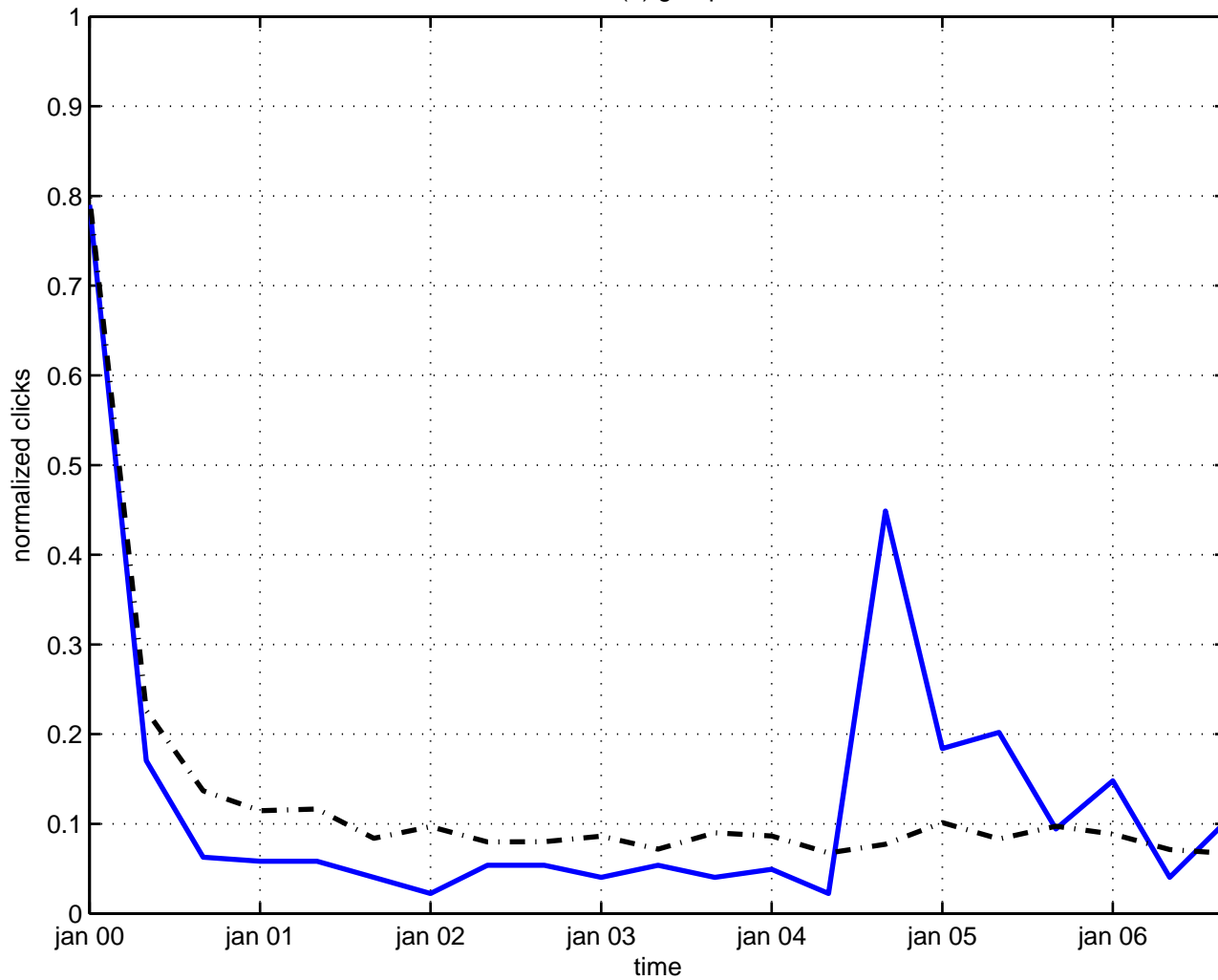
su(5) group
