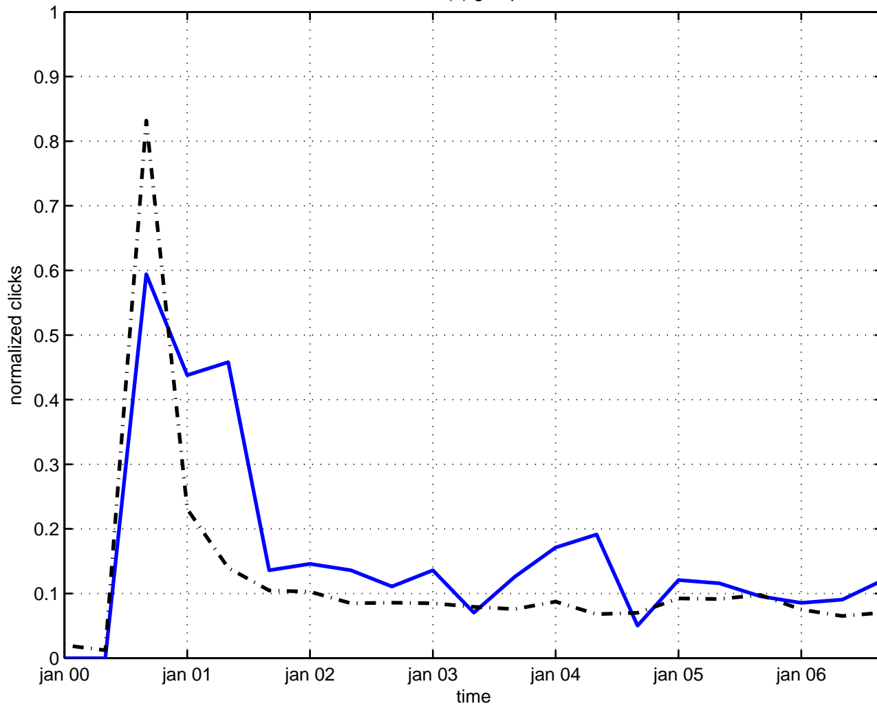
su(4) group
