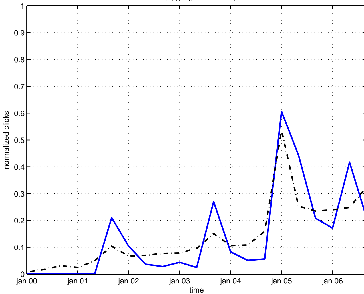
su(4) gauge field theory
