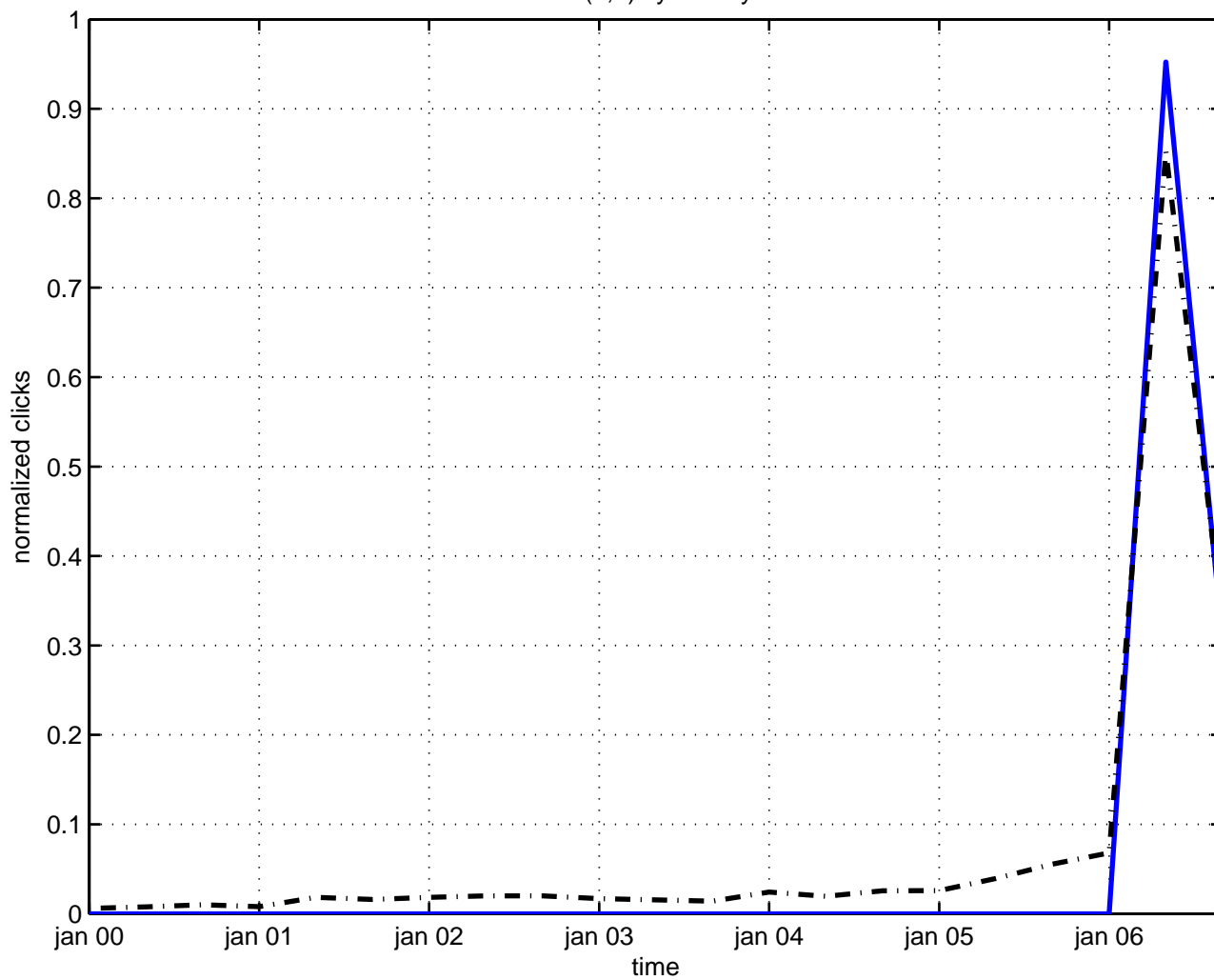
su(3,2) symmetry
