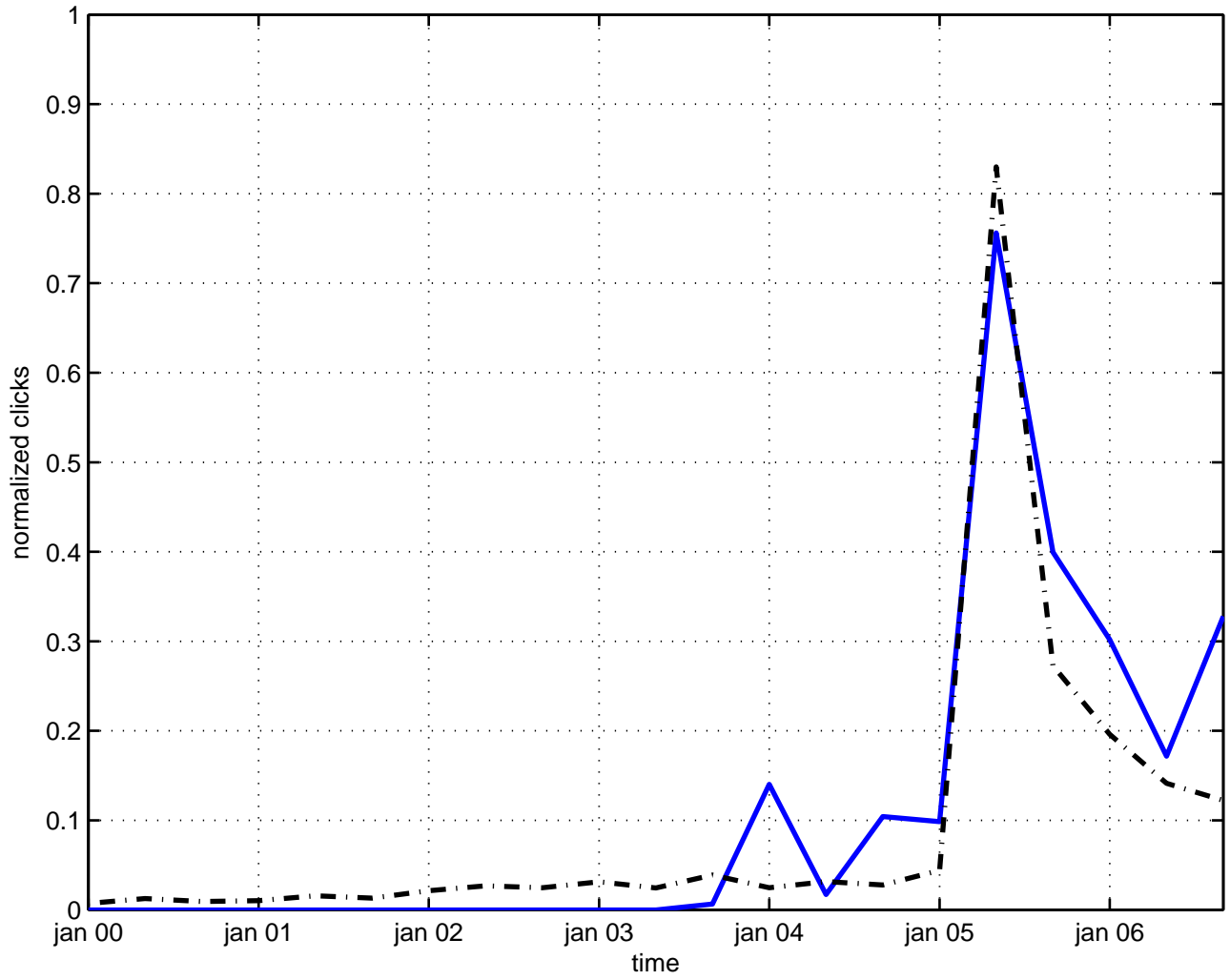
su(3) x su(3) symmetry
