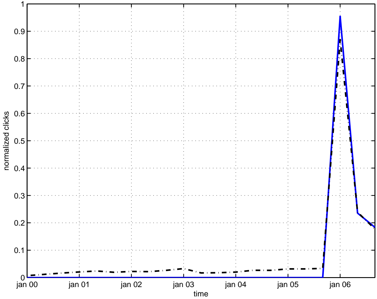
su(3) orientifold
