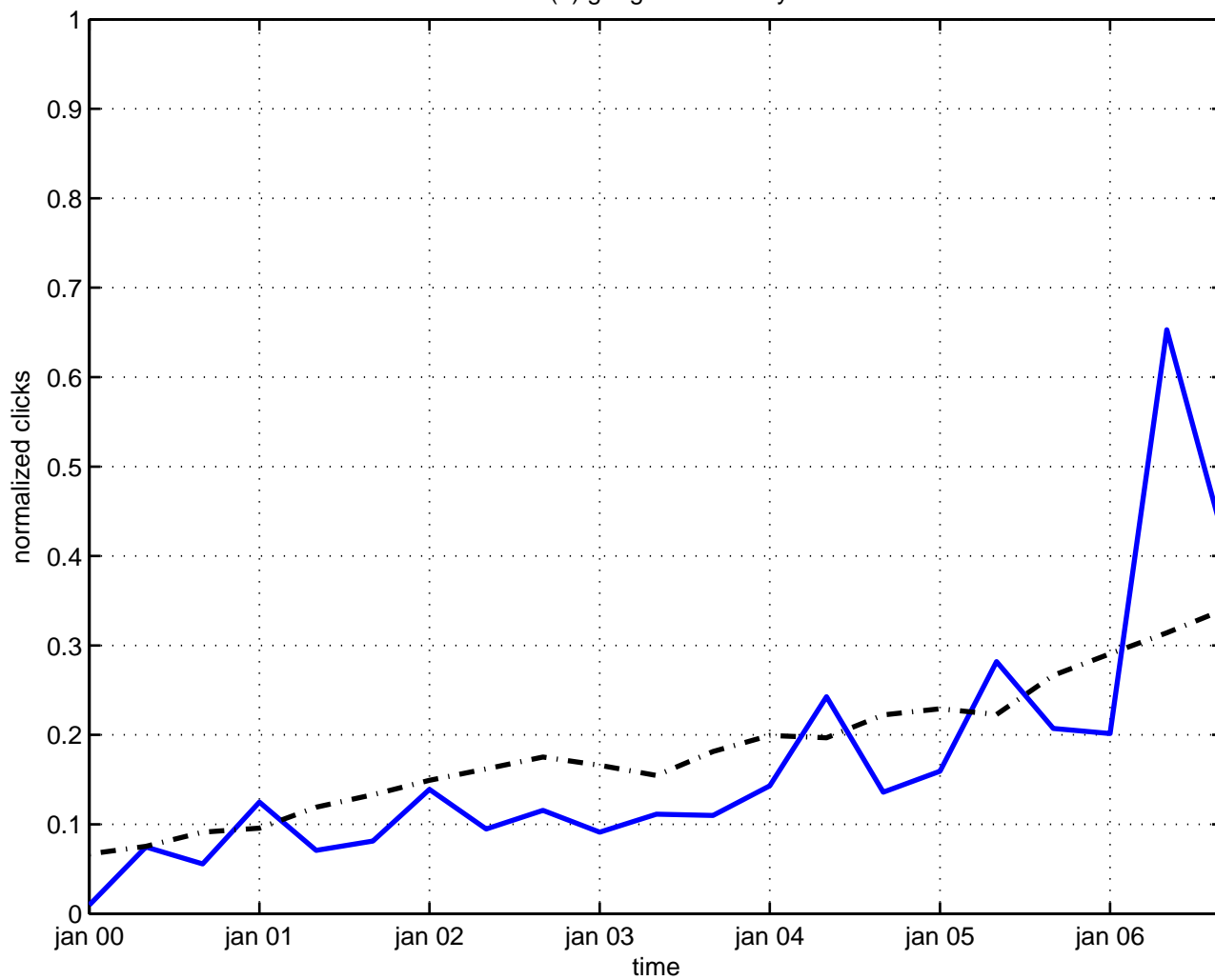
su(3) gauge field theory
