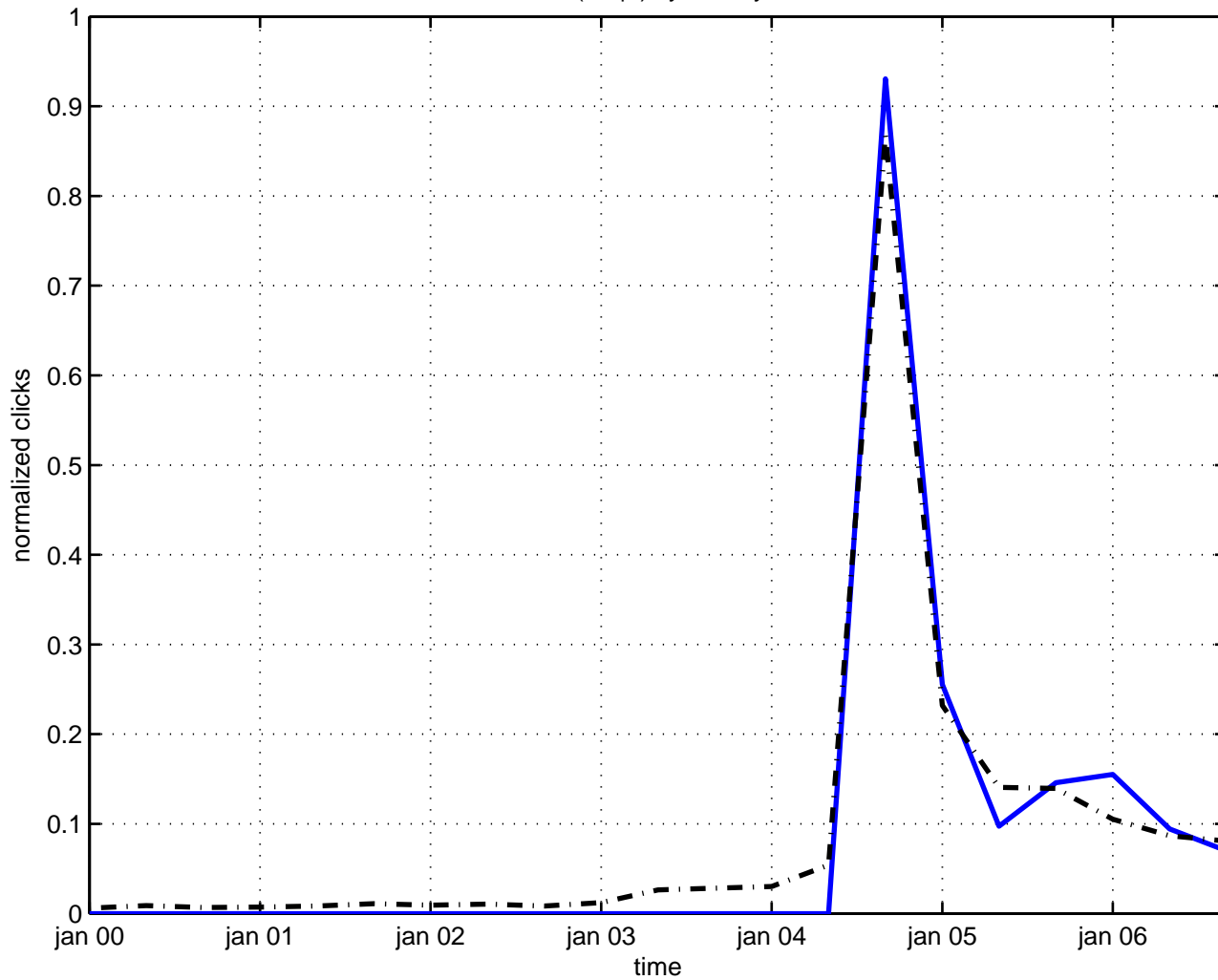
su(2,2|n) symmetry
