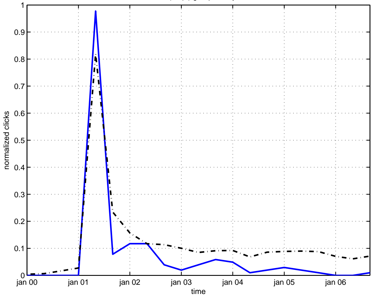
su(2,2|1) group theory
