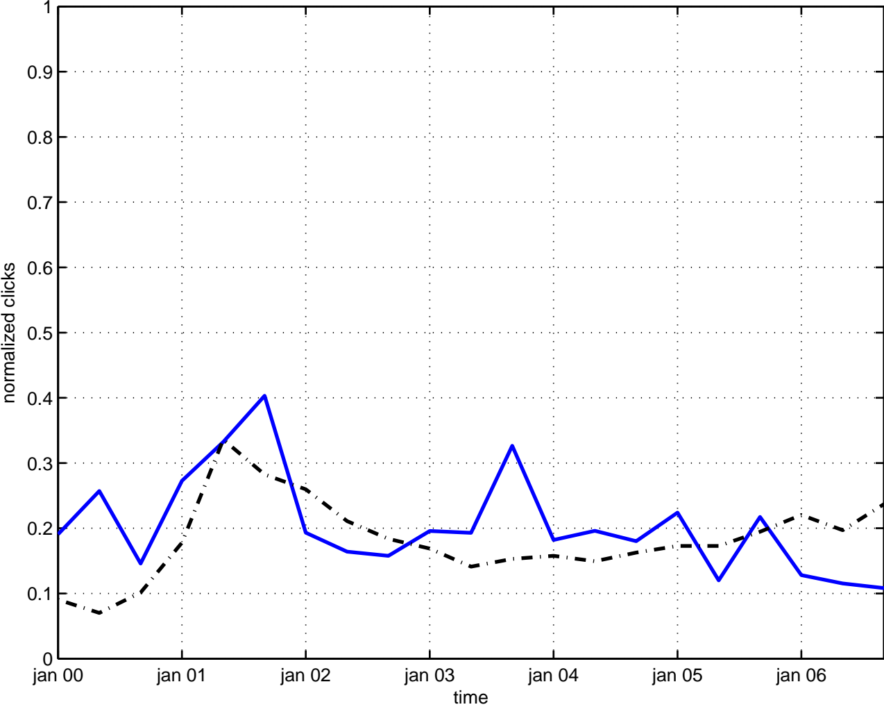
su(2) wess-zumino-witten model
