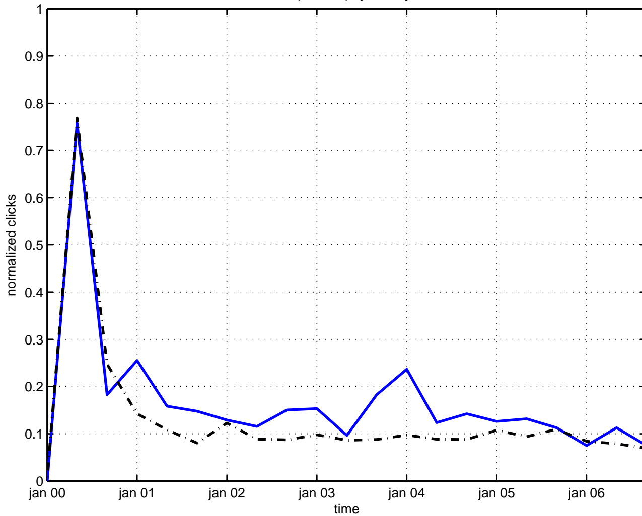
su(16,16/1) symmetry
